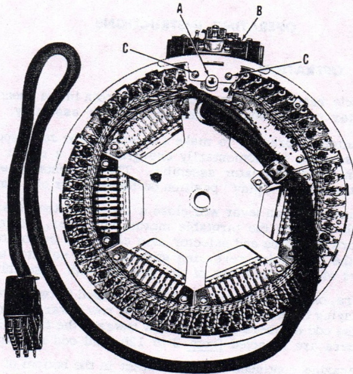
FIG. 1 SELECTOR UNIT
