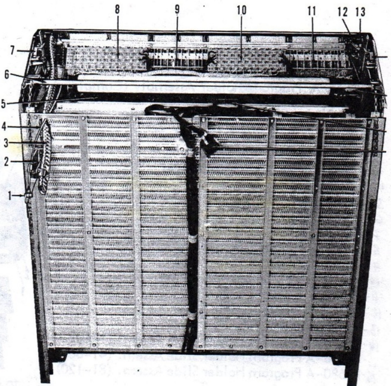
No. 19665-A Door Assembly (Rear View)
