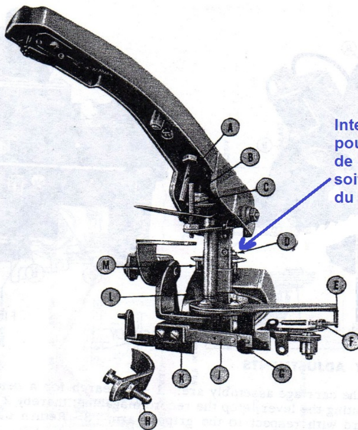
FIG. 4 TONE ARM ASSOCIATED PARTS
