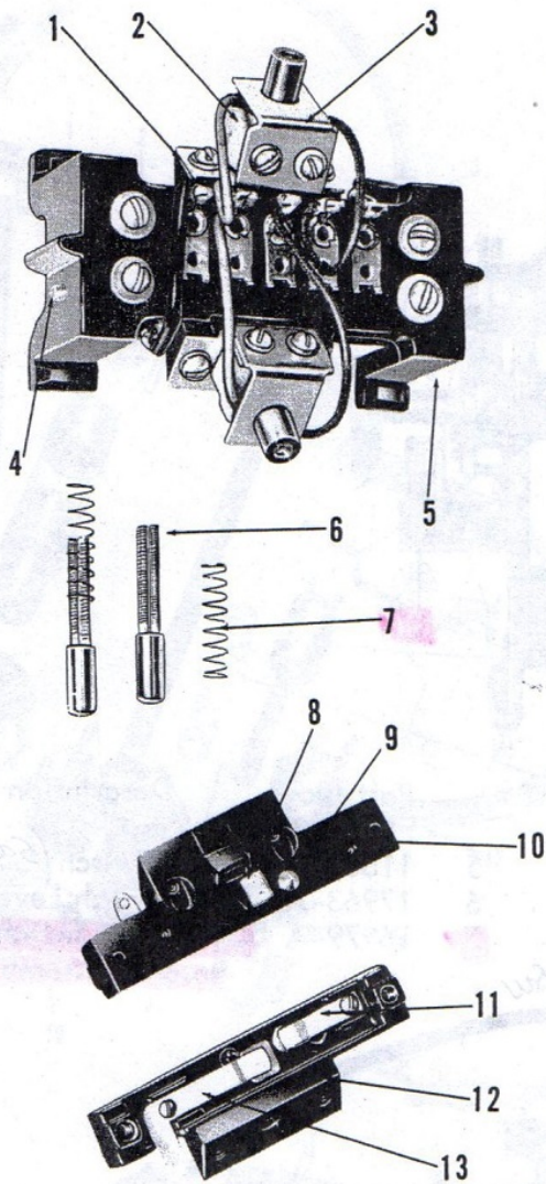
No. 19566-A Record Magazine Assembly
