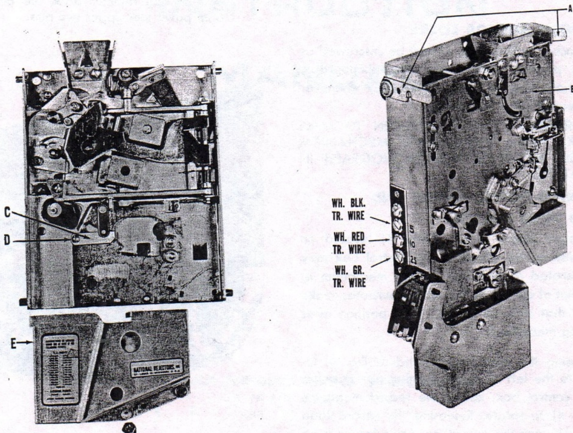
FIG. 6 SLUG REJECTOR
