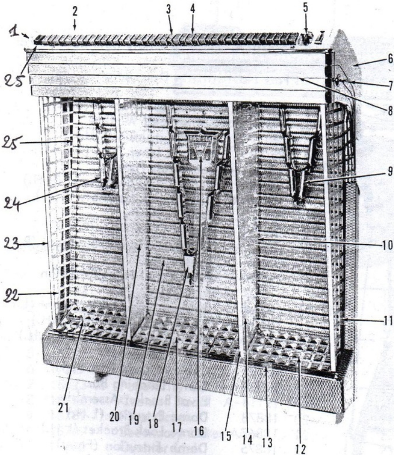
No. 19665-A Door Assembly (Rear View)
